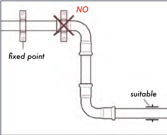
Fig. 15 Pipe fixing: fixed point on fitting: wrong
