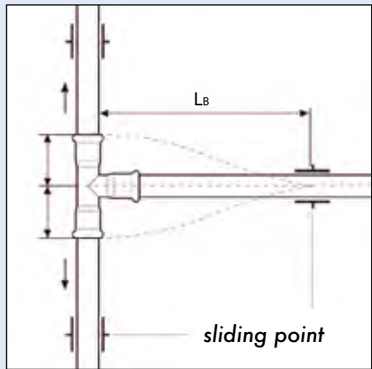
Fig. 11 T-shaped branch Maximum distance between fixing point
